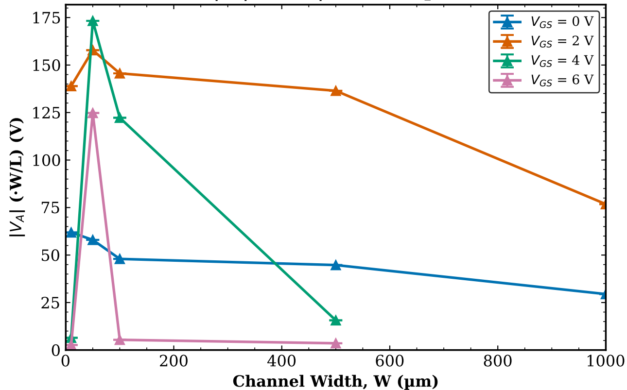
TFT2 Transistor 2 |V_A| vs W | L = 160 \mu\text{m}
